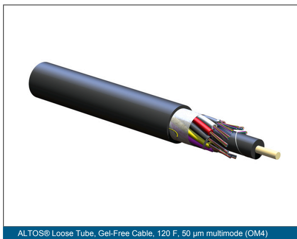
ALTOS® Loose Tube, Gel-Free Cable, 120 F, 50 µm multimode (OM4)
