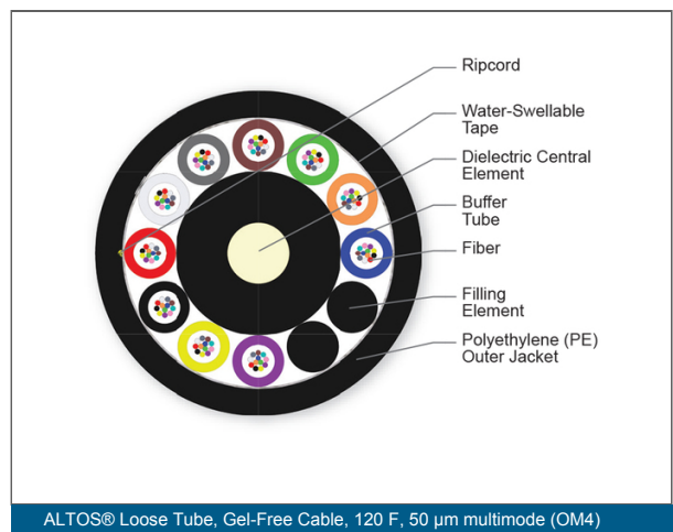
ALTOS® Loose Tube, Gel-Free Cable, 120 F, 50 µm multimode (OM4)
